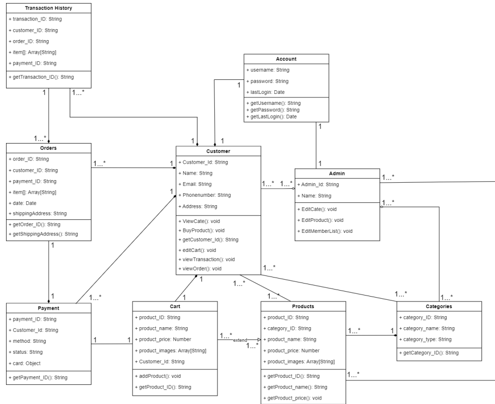
Image 34. Class diagram
